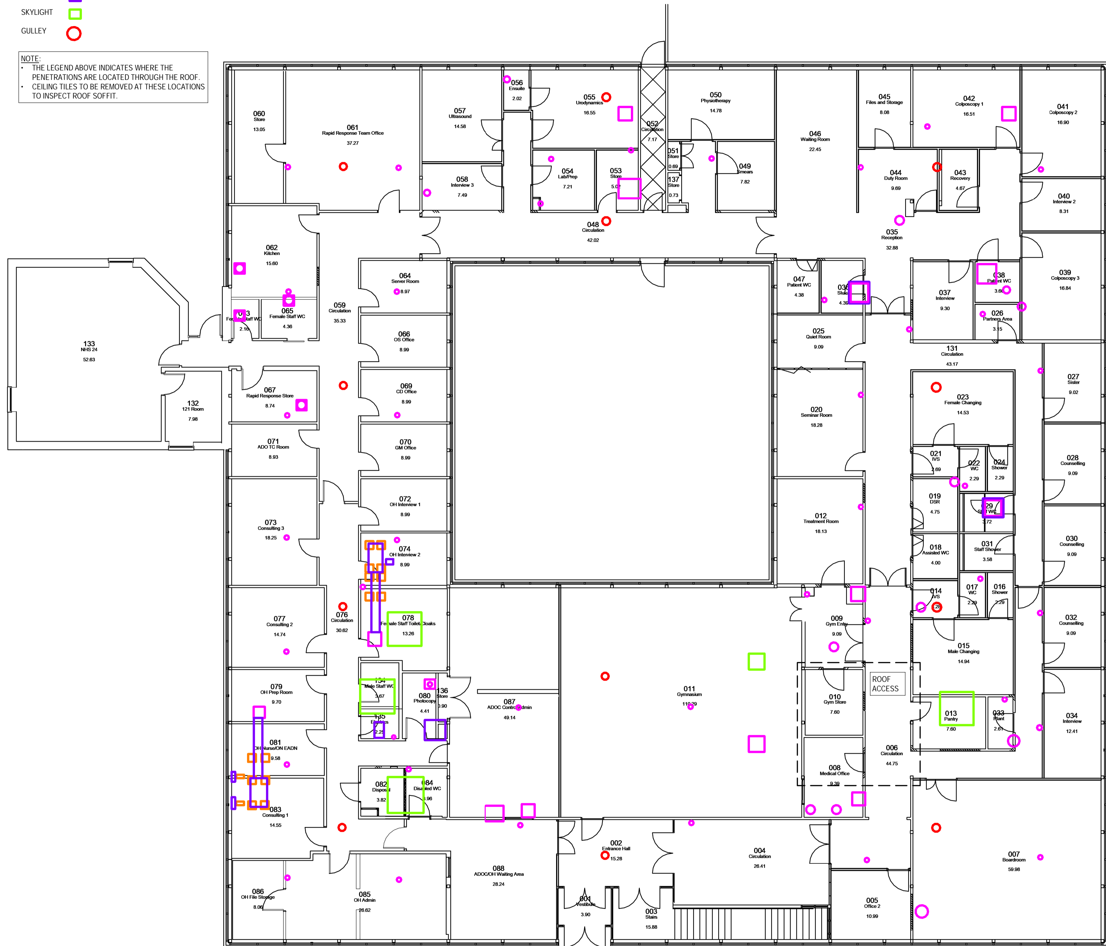
PROPOSED GROUND FLOOR LAYOUT
